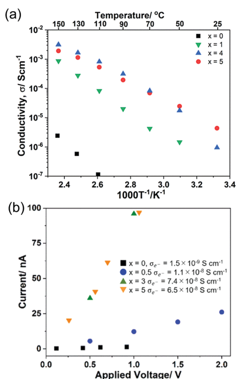
Fig. 4 Temperature dependence of ionic conductivity (a) and I - V correlation (polarized electronic current) (b) of (100 - x)\text{Li}_2\text{S} - x\text{AlI}_3 .
