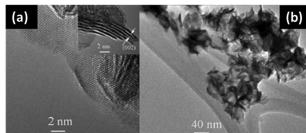
Fig. 5 HRTEM image of MoSe 2 prepared by a hydrothermal method. Reprinted with permission from ref. 52 [H. Tang, K. Dou, C.-C. Kaun, Q. Kuang and S. Yang, J. Mater. Chem. A , 2014, 2 , 360–364.]. Copyright The Royal Society of Chemistry.
