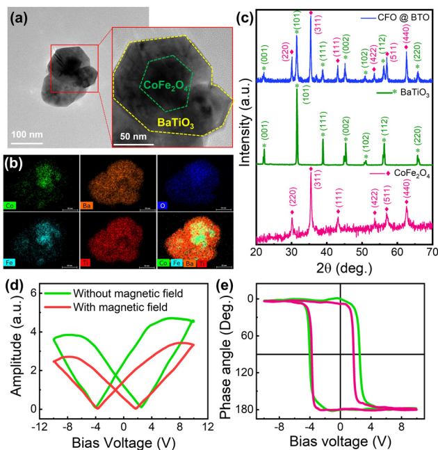
Fig. 1 Characterization of core-shell \text{CoFe}_2\text{O}_4@ \text{BaTiO}_3 MENPs prepared by the sol-gel method. (a) Transmission electron microscopy (TEM) image of the CFO@BTO nanoparticles showing a clear core-shell structure. (b) EDX mapping images of MENPs highlighting the presence of a BTO shell over the CFO core as revealed by the elemental distributions of Co and Fe in the CFO core and Ba and Ti in the BTO shell. (c) X-Ray diffraction patterns of the MENPs, BTO, and CFO (*: BTO phase, \blacklozenge : CFO phase). (d) Local piezoresponse, amplitude voltage butterfly loops, and (e) phase voltage hysteresis loops of the MENPs during ferroelectric and magneto-electric characterization using PFM with and without a magnetic field of 1 kOe.
