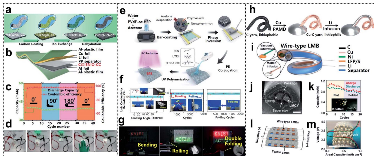
Fig. 8 Foldable lithium-ion batteries. (a) Schematic illustration of fabrication of carbon-coated IE-synthesized NiO nanosheet arrays on CC(C@ENiO-CC). (b) a pouch cell structure based on C@ENiO-CC. (c) cycling performance of the cell in bending states and (d) optical images of the cell lighting up LED bulbs in flat and bended states. Reproduced from ref. 107. Copyright 2021, Wiley-VCH. (e) Schematic procedure for preparing porous PVDF-co-HFP intertwined SPE, (f) ionic conductivity under several deformation processes and (g) optical images of LEDs lit by LFP/40-INSPE 1 : 2/Li with bending, rolling, and double-folding. Reproduced from ref. 109. Copyright 2020, American Chemical Society. (h) Fabrication process of a lithium-metal composite yarn (LMCY), (i) structural design of the wire-type lithium-metal batteries (LMBs), (j) sectional SEM image of the as-fabricated wire-type LFP||LMCY battery, (k) capacity retention of the battery in flat and folded states, and inset shows the optical image of powered LEDs by the knotted batteries, (l) schematic image of the battery textile and (m) voltage profiles of the battery textile, the inset shows the optical image of the as-fabricated battery textile. Reproduced from ref. 111. Copyright 2021, Wiley-VCH.
