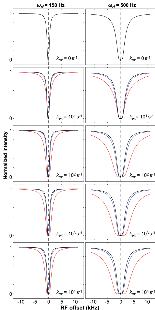
Fig. 8 Simulated DEST profiles for a two-site exchange equilibrium between the NMR-visible ( p_A = 0.95 and R_2^A = 10 \text{ s}^{-1} ) and NMR-invisible ( p_B = 0.05 ) states over a range of k_{ex} values (0 to 10^4 \text{ s}^{-1} , top to bottom). R_2^B was set to 100 (blue line) or 1000 \text{ s}^{-1} (red line) to simulate adsorption to a small or large NP, respectively. The DEST curve simulated at k_{ex} = 0 \text{ s}^{-1} (corresponding to the data obtained in the absence of NP) is colored black. The saturation field strengths are 150 and 500 Hz for the left and right panels, respectively. Note that the DEST experiment is most efficient in detecting ligand-NP adduct with large R_2^B that exchange slowly with the desorbed state ( k_{ex} \ll R_2^B - R_2^A ). In the fast exchange limit, the shape of the DEST profile is no longer dependent from k_{ex} .
