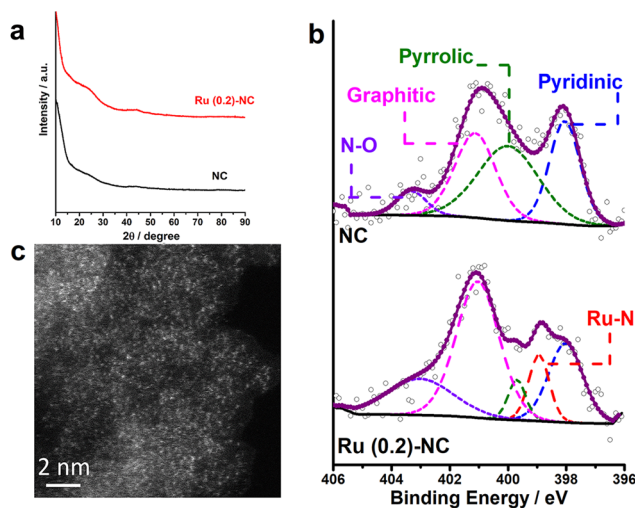
Fig. 1 (a) XRD patterns and (b) high-resolution N1s spectra of Ru (0.2)-NC and pristine NC. (c) HAADF-STEM image of Ru (0.2)-NC.
