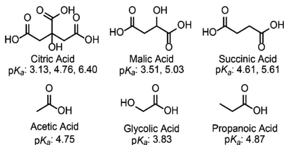
Scheme 1 Fully protonated structures and \text{pK}_a s of the acids discussed in this study.
