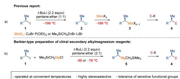
Scheme 1 (a) Previous preparation of chiral secondary alkyl organometallics of type 3 via I/Li-exchange and subsequent transmetalation at -100\text{ }^\circ\text{C} ; (b) Barbier-type preparation of chiral secondary alkylmagnesium reagents (5) via I/Li-exchange and in situ transmetalation with \text{Me}_3\text{SiCH}_2\text{MgCl} at -50\text{ }^\circ\text{C} or -78\text{ }^\circ\text{C} .
