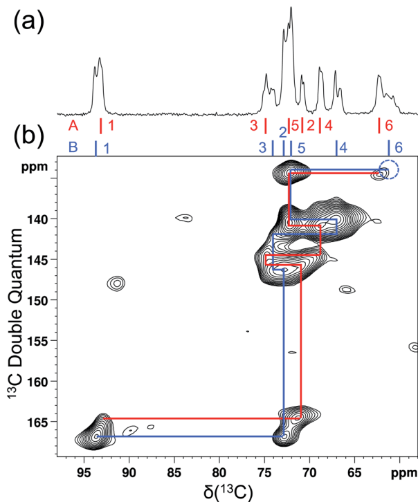
Fig. 8 Natural abundance ^{13}\text{C} (a) 1D CPMAS and (b) 2D refocused INADEQUATE NMR spectra of [2\text{-}^{17}\text{O}]\text{-}\alpha\text{-D-glucose} doped with 10% (w/w) Cu-EDTA. The dotted blue circle indicates the absence of the C6B signal due to its relatively short T_2 (3.7 ms). Both spectra were obtained at 18.8 T with a Bruker 3.2 mm CPMAS CryoProbe. The sample spinning frequency was 15 kHz. Data acquisition parameters are: (a), 1D CP/MAS, contact time 3 ms, recycle time 3.7 s, 16 transients; (b), 2D refocused INADEQUATE, recycle delay 2 s, 1536 transients per t_1 , 34 t_1 increments, J-evolution period of 3.99 ms, total experimental time 30 h.
