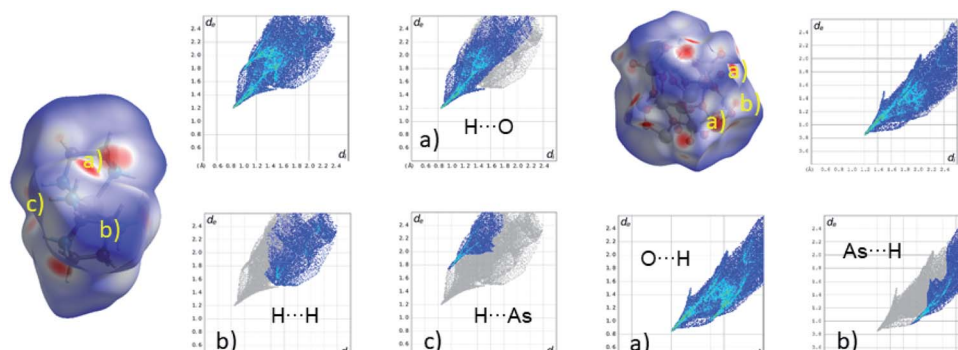
Fig. 4 Hirshfeld surface and fingerprint plots of [Ni(en) 3 ] 2+ dications (left) and the polyanionic unit [V 6 As 8 O 26 ] 4- (right) in the structure of 1. The intermolecular interactions are indicated as red areas on the Hirshfeld surfaces and the distinct interactions are shown in the four fingerprint plots right next to the species. The letters on the Hirshfeld surface (a, b and c) refer to the according letter in the fingerprint plot.
