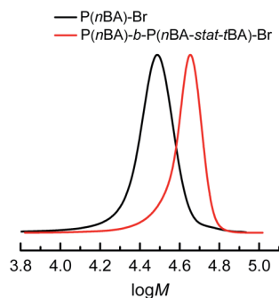
Fig. 5 Molecular weight distribution of P( n BA) _{288} -Br macroinitiator ( M_n = 37.0 kDa and \bar{D} = 1.11 , \text{conv}_{n\text{BA}} = 83\% ) and P( n BA) _{288} - b -P( n BA) _{40} - stat -tBA _{56} )-Br copolymer ( M_n = 50.6 kDa and \bar{D} = 1.06 , \text{conv}_{t\text{BA}} = 25\% , \text{conv}_{n\text{BA}} = 94\% ) produced by PGE eATRP of n BA and n BA + tBA at T = 45^\circ\text{C} in DMF + 0.1 M \text{Et}_4\text{NBF}_4 . tBA was added after 1 h of n BA polymerization under the following conditions: n\text{BA}/\text{EBiB}/\text{Cu}(\text{OTf})_2/\text{Me}_6\text{TREN}/\text{Et}_4\text{NBr} = 349/1/0.1/0.3/0.1 , C_{n\text{BA}} = 3.49 M.
