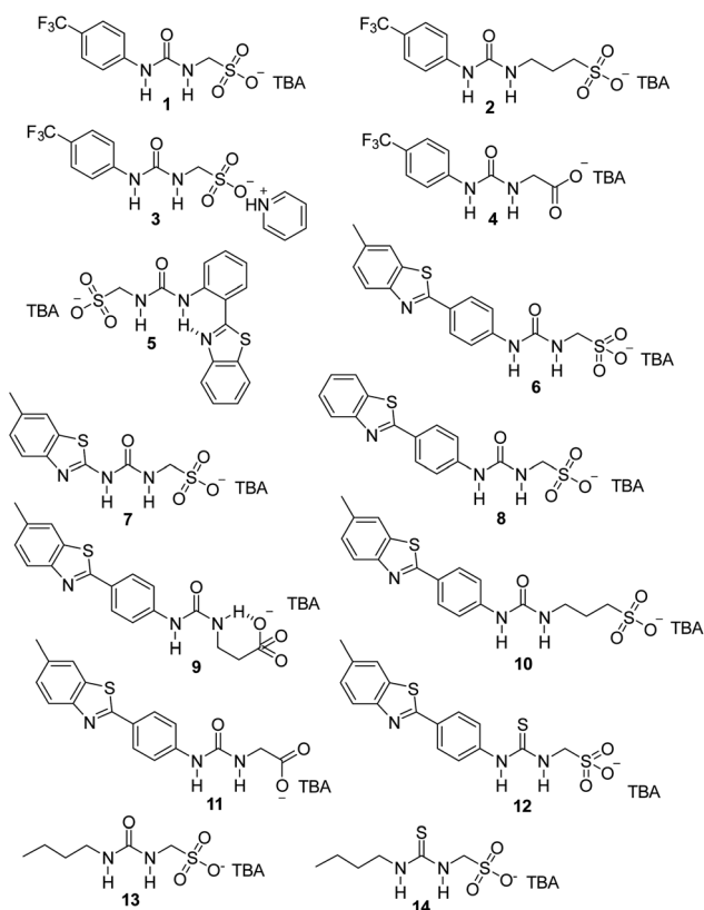
Fig. 1 Chemical structures of SSAs 1–14. TBA = Tetrabutylammonium.
