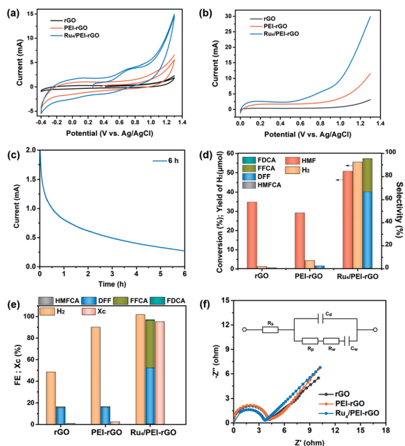
Fig. 5 (a) CV and (b) LSV curves of rGO, PEI-rGO and Ru 4 /PEI-rGO electrocatalysts. (c) The i - t response curve of Ru 4 /PEI-rGO at 0.94 V vs. Ag/AgCl for 6 h. The conversion of HMF, the selectivity of liquid products and the yield of H 2 (d) and FE (e) of products for rGO, PEI-rGO and Ru 4 /PEI-rGO electrocatalysts upon bulk electrolysis at 0.94 V vs. Ag/AgCl for 6 h at room temperature. (f) Nyquist plots for rGO, PEI-rGO and Ru 4 /PEI-rGO in 5 mM HMF (0.5 M pH = 6 HAC/NaAc) at 0.94 V vs. Ag/AgCl and the equivalent circuit diagram.
