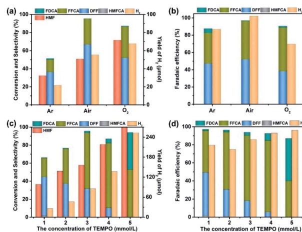
Fig. 6 The effects of the reaction atmosphere (a and b) and concentration of TEMPO (c and d) on the electrocatalytic activities of Ru 4 /PEI-rGO.
