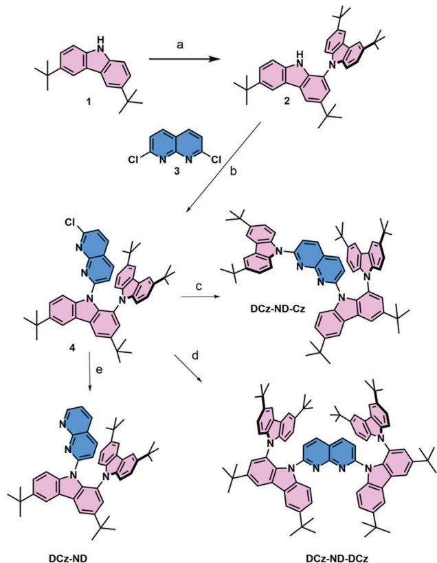
Scheme 1 Reagents and conditions: (a) [\text{Ru}(\text{p-cymene})\text{Cl}_2]_2 , dppe, \text{Cu}(\text{OAc})_2 , PhCl, 1,1,2,2-tetrachloroethylene, AcOH, \text{O}_2 , 150 °C, 82%; (b) 2 , 3 , n -BuLi, THF, 80 °C, 86%; (c) 3,5-di- tert -butylcarbazole, NaH, THF, 80 °C, 88%; (d) NaH, THF, 40%; and (e) \text{Pd}(\text{OAc})_2 , \text{Bu}_4\text{NBr} , DMF, i PrOH, 115 °C, 36%.
