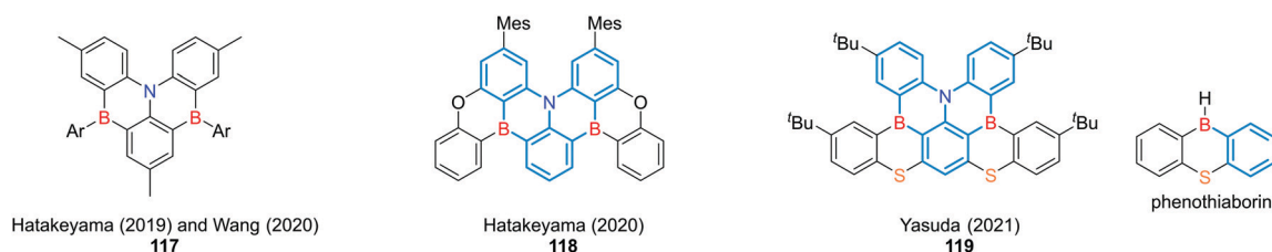
Fig. 35 BNB-doped PAHs for MR-TADF.
