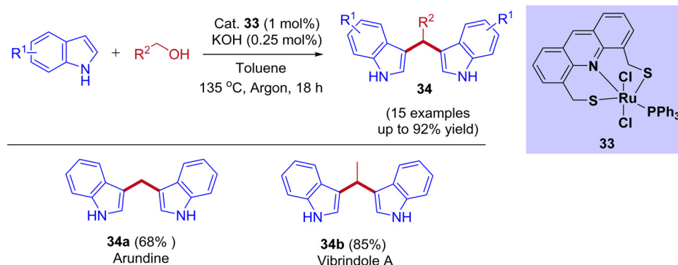
Scheme 16 Ru-SNS pincer-catalyzed synthesis of bis(3-indolyl)phenylmethane derivatives.
