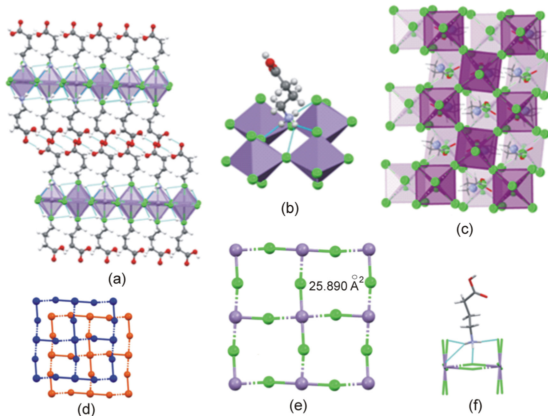
Fig. 7 (a) Packing diagram of structure C4MnCl , viewed down the b -axis, parallel to the inorganic layers. (b) Gauche bond in cation, and hydrogen bonding interactions in structure C4MnCl . Hydrogen bonds are indicated by blue dashed lines. (c) View of structure C4MnCl perpendicular to the inorganic layer, showing two consecutive, staggered inorganic layers, and the tilting of the polyhedra relative to each other. (d) Staggered arrangement of two consecutive inorganic layers, viewed perpendicular to the inorganic layer. Terminal halide ions are excluded for clarity. The top layer is shown in blue, and the bottom layer in orange. (e) 2D inorganic grid created by metal ions and bridging halide ligands. (f) Penetration of ammonium group into cavity created by metal ions and bridging and terminal halide ligands.
