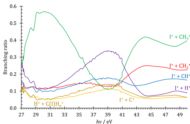
Fig. 4 Double ionization branching ratios plotted for the observed ion pairs as detected by PEPICO in the 27–50 eV photon energy range.
