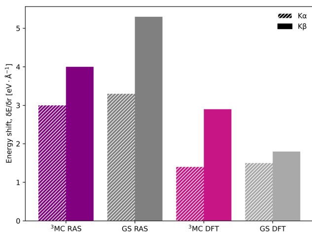
Fig. 6 Energy shifts ( \delta E_{\text{max}}/\delta r ) in \text{eV } \text{\AA}^{-1} for K \alpha (striped bars) and K \beta (solid bars) spectra, calculated with RAS and 1-DFT BP86 for ^3\text{MC} and GS electron configurations.
