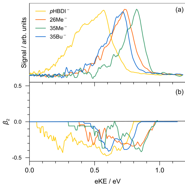
Fig. 2 Photoelectron spectroscopy performed at hν = 3.44 eV (360 nm): (a) pHBDI − (yellow), 26Me − (orange), 35Me − (green), and 35Bu − (blue); (b) β 2 parameters (±0.1 uncertainty) associated with the photoelectron spectra in (a).
