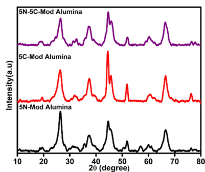
Fig. 9 XRD profile of spent 5Ni-mod alumina, 5Co-mod alumina, and 5Ni-5Co-mod alumina catalysts.
