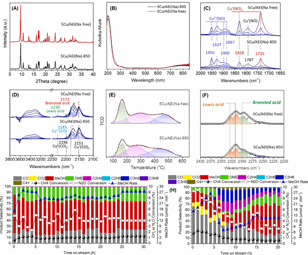
Fig. 13 (A) XRD patterns and (B) UV-vis spectra of 5Cu/AEI(Na)-850 and 5Cu/AEI(Na free). In situ FT-IR spectra of adsorbed (C) NO (5–120 Pa) and (D) CO (5–1000 Pa) on Cu ion-exchanged AEI-type zeolites at 153 K. (E) \text{NH}_3 -TPD profiles. (F) In situ FT-IR spectra of adsorbed \text{CD}_3\text{CN} species on Cu ion-exchanged AEI-type zeolites at room temperature. Catalytic performance of (G) 5Cu/AEI(Na)-850 and (H) 5Cu/AEI(Na free) in the MTM reaction. Reaction conditions: 100 mg catalysts; \text{CH}_4/\text{N}_2\text{O}/\text{H}_2\text{O}/\text{Ar} = 10/10/2/3 \text{ mL min}^{-1} ; WHSV = 15\,000 \text{ mL h}^{-1} \text{ g}_{\text{cat}}^{-1} ; 623 K. Reprinted from ref. 62 with permission from Elsevier, copyright 2023.
