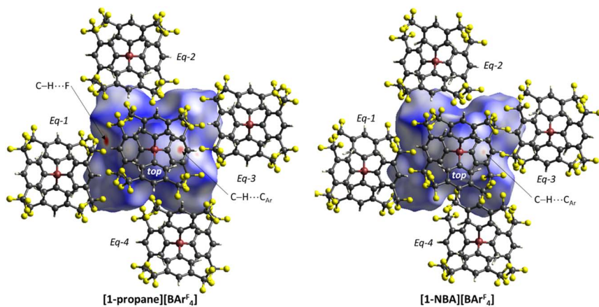
Fig. 3 Hirshfeld surfaces mapped over d_{\text{norm}} for [1-NBA] + and [1-propane] + within the octahedral arrays of neighbouring [\text{BARF}_4]^- anions with the anion labelling system indicated. Views are taken from above the 'top' anion looking down the \text{B}_{\text{top}} \cdots \text{Rh} \cdots \text{B}_{\text{bottom}} axis; the 'bottom' anion is obscured by the cation surface.
