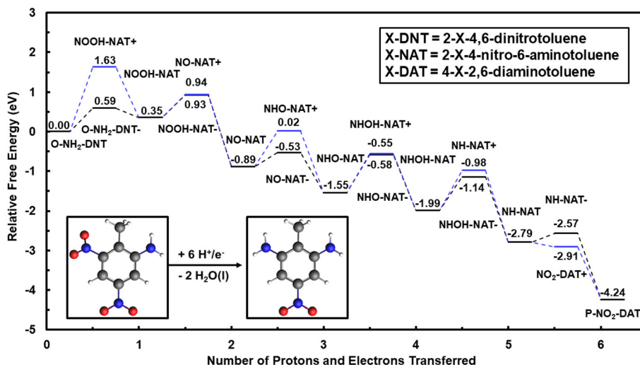
Fig. 2 Reaction energy diagram for outer-sphere electrochemical reduction of O\text{-NH}_2\text{-DNT} to P\text{-NO}_2\text{-DAT} in the solution phase, calculated using the G16 code and IEFFPCM solvation model. Reduction proceeds by reducing the second ortho \text{NO}_2 group to the methyl group of TNT. Energies are relative to O\text{-NH}_2\text{-DNT} in the solution phase at 0 V-NHE and pH = 0. Water molecules formed during the TNT reduction are not shown for clarity purposes. Black lines represent reduction steps initiated by uncoupled electron transfer followed by proton transfer. Blue lines represent reduction steps initiated by uncoupled proton transfer followed by electron transfer. Atom colors are presented as grey: C, white: H, blue: N, and red: O.
