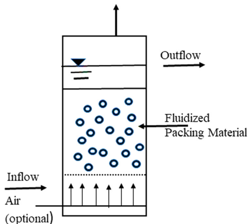
Fig. 6 Fluidized bed biofilm reactor. 135
