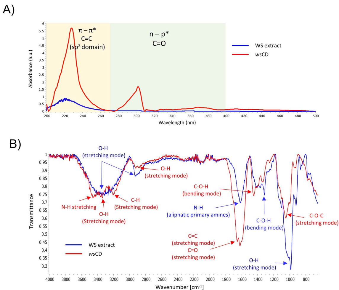
Fig. 2 Chemical structure and surface functional group analysis. (A) Chemical structure analysis of WS extract and w\text{sCDs} using UV absorption spectroscopy; (B) surface functional group analysis of WS extract (blue) and w\text{sCDs} (red) using Fourier transform infrared spectroscopy.
