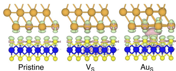
Fig. 4 Electron density difference (EDD) maps of the pristine, V_{\text{S}} and \text{Au}_5 interfaces in the vicinity of the contact area. Green colour corresponds to electron loss, whereas mauve colour to electron enrichment. The isovalue was set to 0.002 \text{ eV } \text{\AA}^{-3} .
