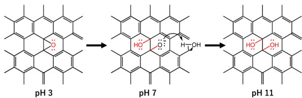
Scheme 1 Illustration of the pH-dependent functional groups change in GO.
