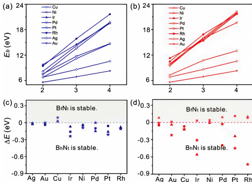
Fig. 3 Binding energies as a function of BN clusters terminated with (a) N and (b) B atoms. The difference in formation energy between B_nN_t and B_tN_n of (c) N and (d) B terminated BN clusters. Squares, stars, and triangles represent the cluster size of 2, 3, and 4, respectively. 180
