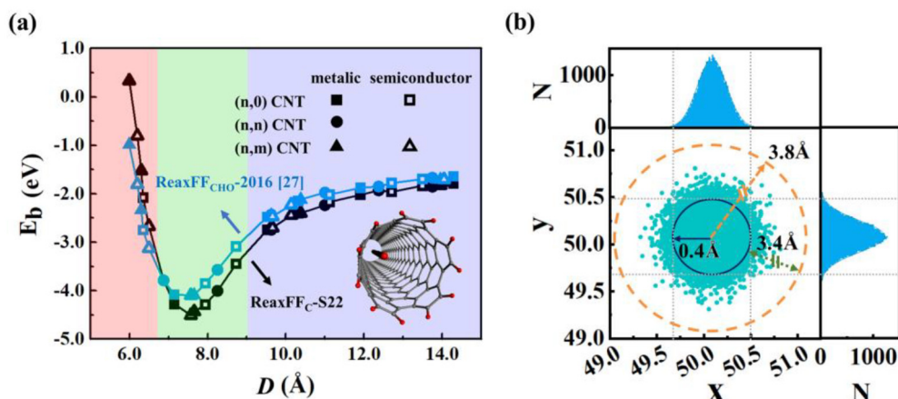
Fig. 7 (a) Binding energies of C_{16}H_2 chain inside finite CNTs with various diameters and chirality calculated by ReaxFF CHO-2016 27 and ReaxFF C-S22 , respectively. The inset is the schematic model of a C_{16}H_2 chain inside a finite (6, 5) CNT. (b) The projected positions of all C atoms of C_{16}H_2 chain at every MD step and the corresponding histogram of probability distribution of x - and y -coordinates.
