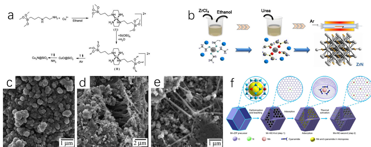
Fig. 3 (a) Synthetic route of \text{Cu}_3\text{N}@\text{SiO}_2 nanocomposites by sol-gel method. 23 Copyright 2011, Royal Society of Chemistry; (b) synthetic route of \text{ZrN} NPS by urea glass method. 24 Copyright 2020, Springer Nature. SEM images of solvothermal products NiN (c), FeN (d), and MnN (e). 25 Copyright 2009, American Chemical Society; (f) synthetic route of the atomically dispersed Mn-N-C catalysts by impregnation adsorption method. 27 Copyright 2018, Springer Nature.
