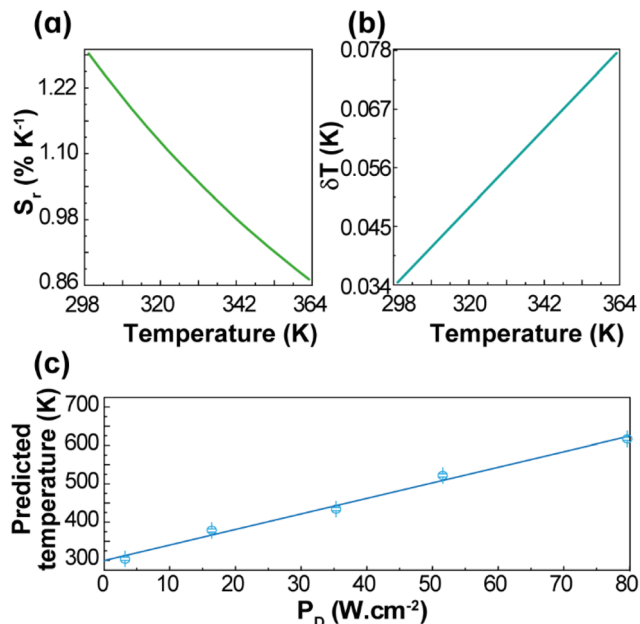
Fig. 4 Temperature dependence of (a) S_r and (b) \delta T of 1 (pellet). (c) Dependence of the predicted temperatures on P_D for 1 (pellet). The line is the best linear fit to the data ( r^2 > 0.985 ).
