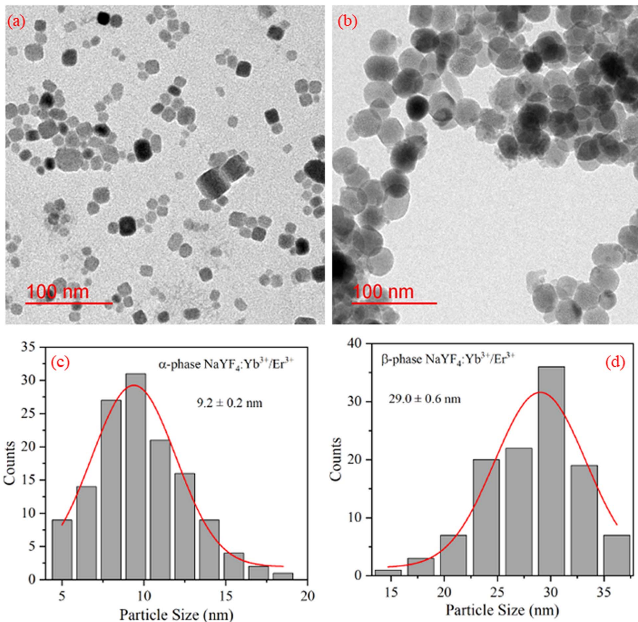
Fig. 2 TEM image of (a) \alpha - \text{NaYF}_4:\text{Yb}^{3+}/\text{Er}^{3+} , (b) \beta - \text{NaYF}_4:\text{Yb}^{3+}/\text{Er}^{3+} nanophosphor. (c) and (d) shows the particle size distribution of \alpha - \text{NaYF}_4:\text{Yb}^{3+}/\text{Er}^{3+} , and \beta - \text{NaYF}_4:\text{Yb}^{3+}/\text{Er}^{3+} nanophosphor, respectively.
