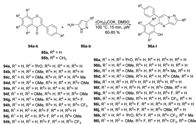
Scheme 33 Synthesis of 5,6-pyrazolo[1,5- a ]pyrimidines 96a–l .
