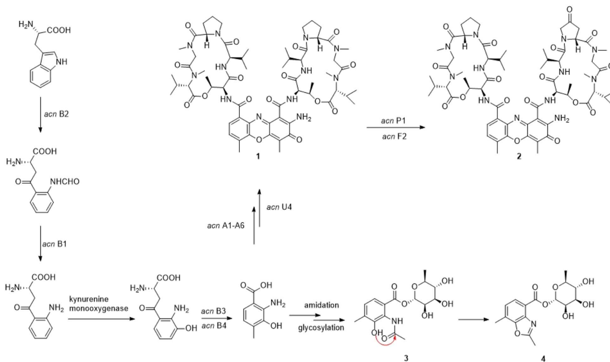
Fig. 6 Proposed biosynthetic pathway of actinrhaters A ( 3 ) and B ( 4 ). acn A1-6 : non-ribosomal peptide synthetase, non-ribosomal peptide synthetase, non-ribosomal peptide synthetase, 3-hydroxy-4-methylanthranilate adenylyltransferase AcnA , 4-MHA carrier protein; acn B1-2 : arylformamidase, tryptophan 2,3-dioxygenase family protein; acn P1-2 : cytochrome P450; acn U4 : hypothetical protein.
