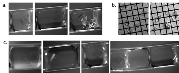
Fig. 5 a. Online camera images of prism parallelepipeds, multiple rhombohedral and clustered crystals (left to right); b. crystals obtained from two sets of 40 slugs, offline camera images of crystals from SS 40–17 crystallisation run, scale grid is 1 mm 2 rhombohedral crystals at the outlet of the KRAIC-G, c. single rhombohedral crystals obtained during NSS ET 55–67 and SS 40–17.
