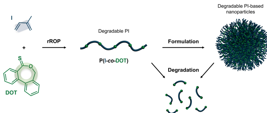
Fig. 1 Synthesis of degradable vinyl polymer nanoparticles via radical ring opening copolymerization (rROP) of dibenzo[ c,e ]oxepane-5-thione (DOT) and isoprene (I) in solution followed by nanoprecipitation.
