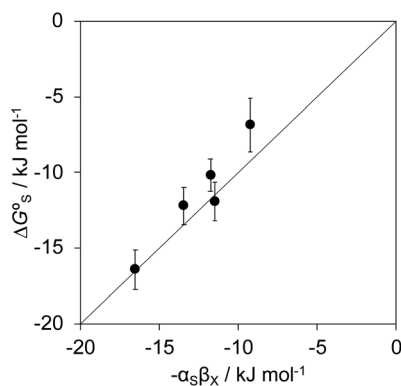
Fig. 13 Experimentally measured stabilisation of complex A in water due to resolution of the guest substituent X ( \Delta G_s^\ddagger ) compared with the calculated free energy change due to formation of a H-bond between X and water ( -\alpha_s\beta_X ). The line corresponds to y = x .
