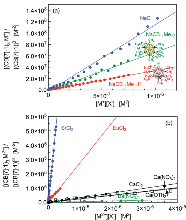
Fig. 7 Plot of [(\text{CB}[7]\cdot 1)_3\text{M}]/[(\text{CB}[7]\cdot 1)_3]^3 as a function of [\text{M}][\text{X}] , for (a) alkali cations M^+ and (b) alkali-earth cations M^{2+} as well as \text{Eu}^{3+} , with linear regressions. Titration affording the best coefficient of determination for each series.
