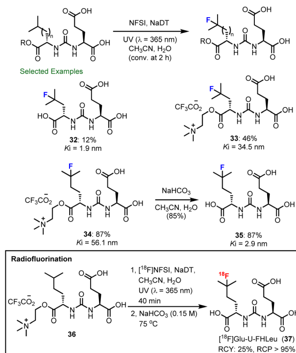
Scheme 9 Accelerated fluorination of choline esters of ZJ-43 and Glu-U-HLeu. PSMA binding of each ligand ( K_f ) was measured by competition assays ( n \geq 3 ) using [ ^{18}\text{F} ]DCFPyL and determined by applying a one-site Fit K_f model using GraphPad Prism (7.04).
