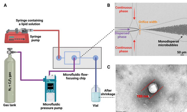
Fig. 1 (A) Schematic of the flow-focusing microfluidic design to generate BNBs. The width of the orifice is 4\ \mu\text{m} , and the height of the microchannels is 20\ \mu\text{m} . (B) Formation of monodisperse MBs at the orifice. (C) TEM image of a BNB after shrinkage with a diameter of 180\ \text{nm} . The BNB's initial diameter before shrinkage was 10.0\ \mu\text{m} . We use a 0.17\ \text{wt}\% \text{C}_3\text{F}_8 gas and a lipid solution with the concentration of 0.50\ \text{mg mL}^{-1} .
