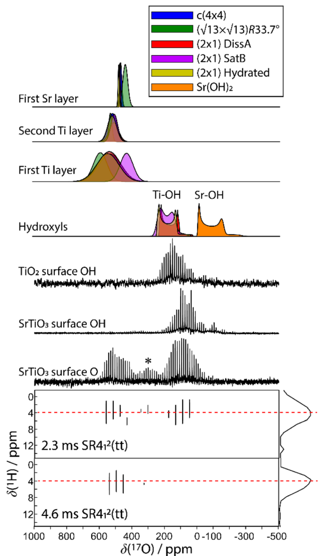
Fig. 5 Experimental (black) D-RINEPT-SR _4^2 (tt) (bottom) 1D and 2D ^{17}\text{O}\{^1\text{H}\} spectra and ^{17}\text{O}\{^1\text{H}\} PRESTO spectra acquired on STO and anatase titania. Simulated spectra are shown on the top corresponding to the parameters calculated using plane-wave DFT for various surface terminations, as indicated on the figure. An asterisk is used to mark the position of a spinning sideband.
