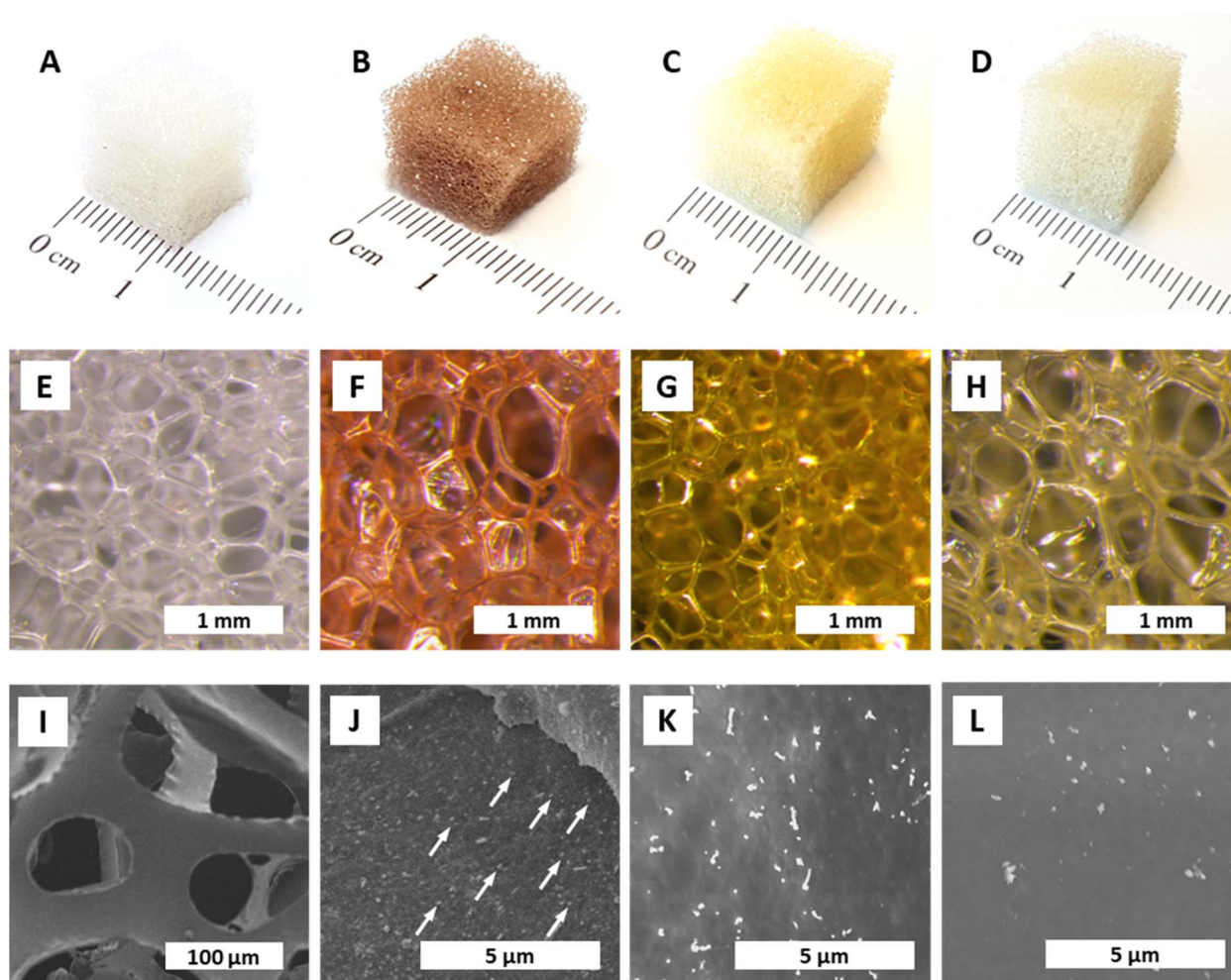
Fig. 1 Aspect and morphology of NPs@PUF. All specimens were synthesized at T_R = 120 °C, t_R = 3 h, and [\text{M}^{*+}] = 0.25 mM. Macroscopic aspect (A–D) and optical micrographs (E–H) of pristine PUF and NPs@PUFs: pristine PUF (A and E), AuNP@PUF (B and F); AgNP@PUF (C and G), PdNP@PUF (D,H). SEM micrographs of pristine PUF(I), and NPs@PUFs: AuNP@PUF (J) with some AuNPs indicated with white arrows; AgNP@PUF (K); and PdNP@PUF (L).
