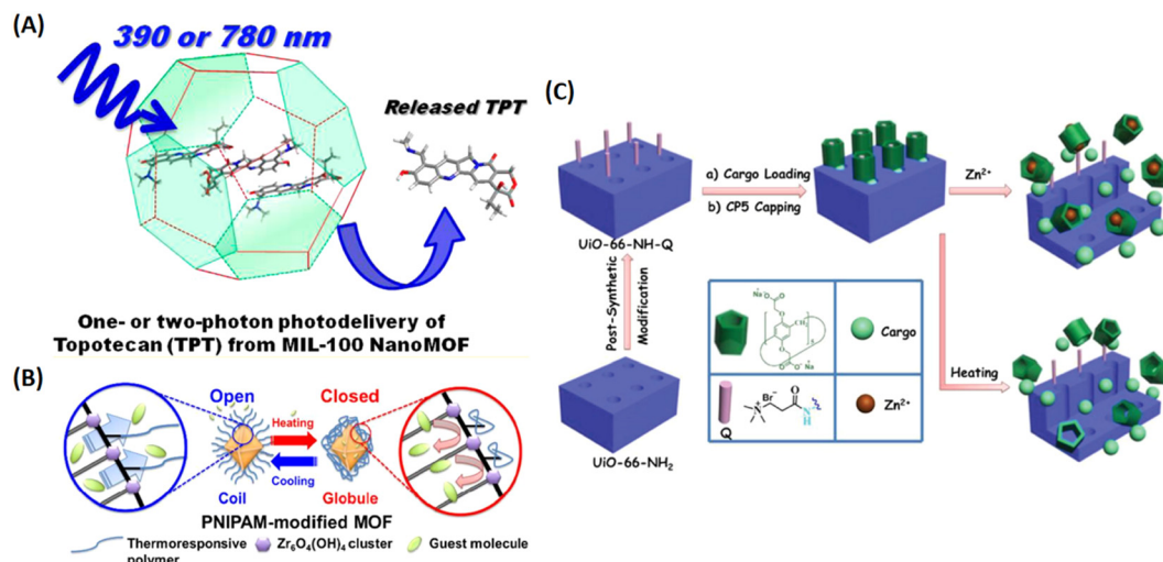
Fig. 7 MIL-100 as a light triggered delivery system for transporting topotecan (TPT). (A) Schematic representation of one- or two-photon photodelivery of TPT from MIL-100. 36 Copyright 2014, Journal of Medicinal Chemistry . (B) Schematic representation of the thermoresponsive controlled release from UiO-66-PNIPAM. 37 Copyright 2015, Chemical Communications (Camb) . (C) Schematic representation of the stimuli-responsive mechanized UiO-66-NH 2 MOFs equipped with positive charged quaternary ammonium salt (Q) encircled by pillar[5]pseudorotaxanes. The mechanized nanoUiO-66-NH 2 MOFs can be operated either by thermal heating or by Zn 2+ competitive binding in regulation of the release of cargo molecules. 25 Copyright 2015, Small .
