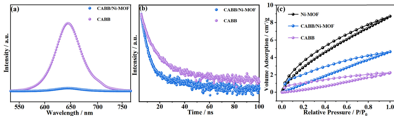
Fig. 9 (a) Steady-state photoluminescence (PL) and (b) time resolved photoluminescence (TRPL) spectra of CABB and the CABB/Ni-MOF hybrid; (c) CO 2 adsorption/desorption curves of CABB NSs, Ni-MOF NSs, and the CABB/Ni-MOF hybrid at 273 K.
