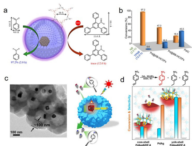
Fig. 6 (a) Schematic illustration of the size-selectivity of a Pd@AB-HCOFs nanoreactor in nitroarene hydrogenation; (b) catalytic activity comparisons of various catalysts. 65 Copyright 2022, American Chemical Society. (c) TEM image and structural model of a core-shell PdAg@ZIF-8 nanoreactor; (d) chemoselective hydrogenation of nitrostyrene with different catalysts. 67 Copyright 2022, American Chemical Society.
