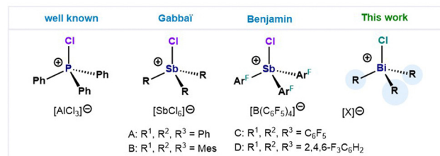
C. This work: Synthesis of high-valent chlorotriarylbismuthonium salts
