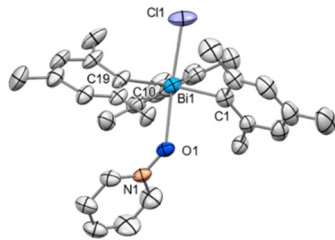
Fig. 5 Solid state structure of 13 . Ellipsoids are drawn at the 50% probability level. H atoms and \text{BAR}^{\text{F}} are omitted for clarity. Selected bond lengths (Å) and angles ( ^\circ ): Bi1–Cl1: 2.507(7), Bi1–O1: 2.404(6), Bi1–C1: 2.229(6), Bi1–C10: 2.226(5), Bi1–C19: 2.236(6), N1–O1: 1.334(8), C1–Bi1–C10: 117.9(2), C1–Bi1–C19: 121.7(2), C10–Bi1–C19: 119.3(2), Cl1–Bi1–O1: 173.5(2), N1–O1–Bi: 136.7(4).
