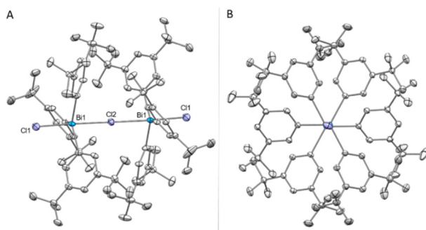
Fig. 4 (A) Solid state structure of 11a . 29 Ellipsoids are drawn at the 50% probability level. H atoms and BARF are omitted for clarity. Selected bond lengths (Å) and angles (°): Bi1–Cl1: 2.4857(7), Bi1–Cl2: 2.80068(13), Bi1–Cl2–Bi1: 180.0, Cl1–Bi1–Cl2: 173.722(17). (B) View along the Cl–Bi–Cl axis.
