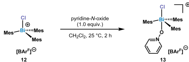
Scheme 3 Synthesis of complex 13 .
