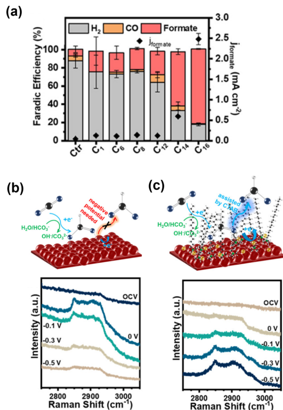
Fig. 10 (a) Dependence of the electrocatalytic CO 2 reduction performance of Cu on the straight-chain alkyl group R of the NR(CH 2 ) 3 Br additive. (b) and (c) In situ Raman spectra of Cu and Cu-CTAB in CO 2 -saturated 0.5 M KHCO 3 under applied potentials, with the schematic illustration of formate formation. Reproduced with permission from ref. 73. Copyright 2020 American Chemical Society.
