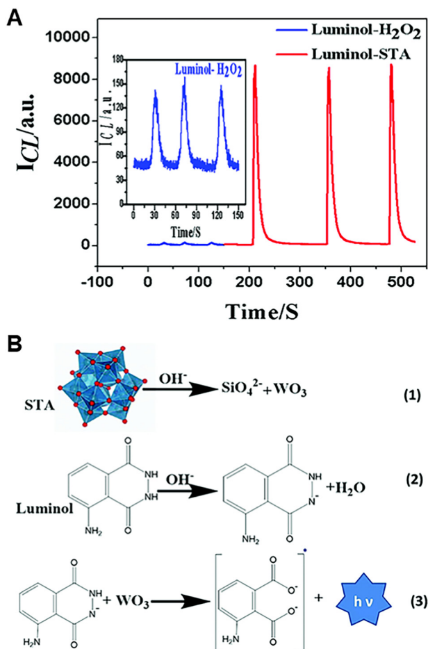
Fig. 3 (A) The relationship between CL intensities and time for the luminol/ \text{H}_2\text{O}_2 system and luminol/STA system [luminol]: 10\ \mu\text{M} ; [STA]: 2\ \text{mM} ; [ \text{H}_2\text{O}_2 ]: 2\ \text{mM} ; pH: 12.0; PMT voltage: -950\ \text{V} . (B) The CL mechanism of the luminol/STA system. Reprinted with permission from ref. 42, Copyright 2020 Royal Society of Chemistry.
