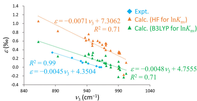
Fig. 4 Relationships between \nu_3 and \epsilon . The horizontal axis shows \nu_3 in units of \text{cm}^{-1} while the vertical axis shows \epsilon in units of \% . The dotted lines are linear regressions and r^2 is the coefficient of determination in each case.
